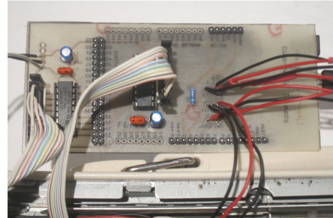
Figure 1: Brain for the knitting machine.
